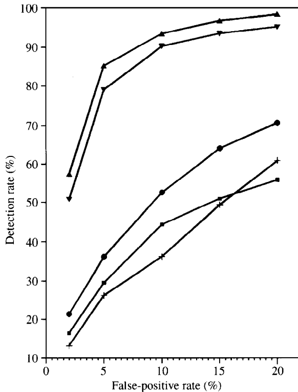
Figure 7 Operator receiver plot if screening was based on maternal age alone (+), maternal serum free \beta -hCG (■) maternal age and maternal serum free \beta -hCG (●), maternal age and fetal nuchal translucency thickness (▼) or maternal age, maternal serum free \beta -hCG and fetal nuchal translucency thickness (▲)
