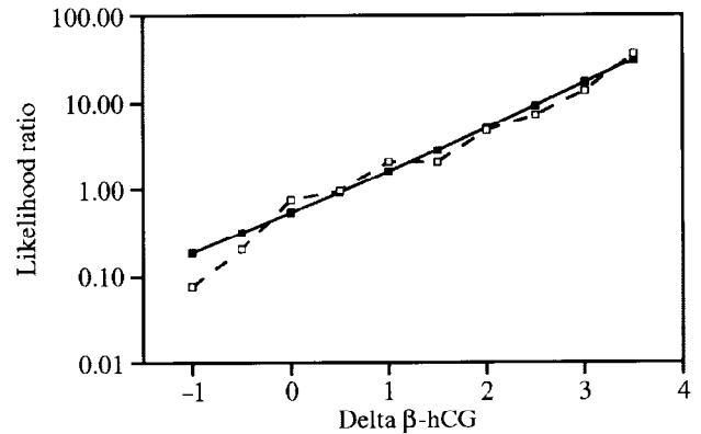
Figure 5 Comparison of likelihood ratios based on actual data (---) to those based on the Gaussian distribution curves (—)
