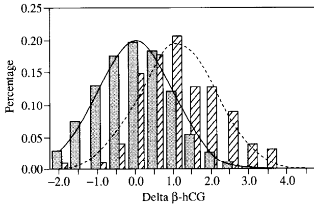
Figure 4 Distribution of delta values for maternal serum free \beta -hCG in 2427 normal (stippled bars) and 102 trisomy 21 pregnancies (hatched bars). For the distribution of delta values in trisomy 21, data from the 61 cases in the present study were combined with those from 41 cases examined previously 3 . Curves assume a Gaussian distribution
