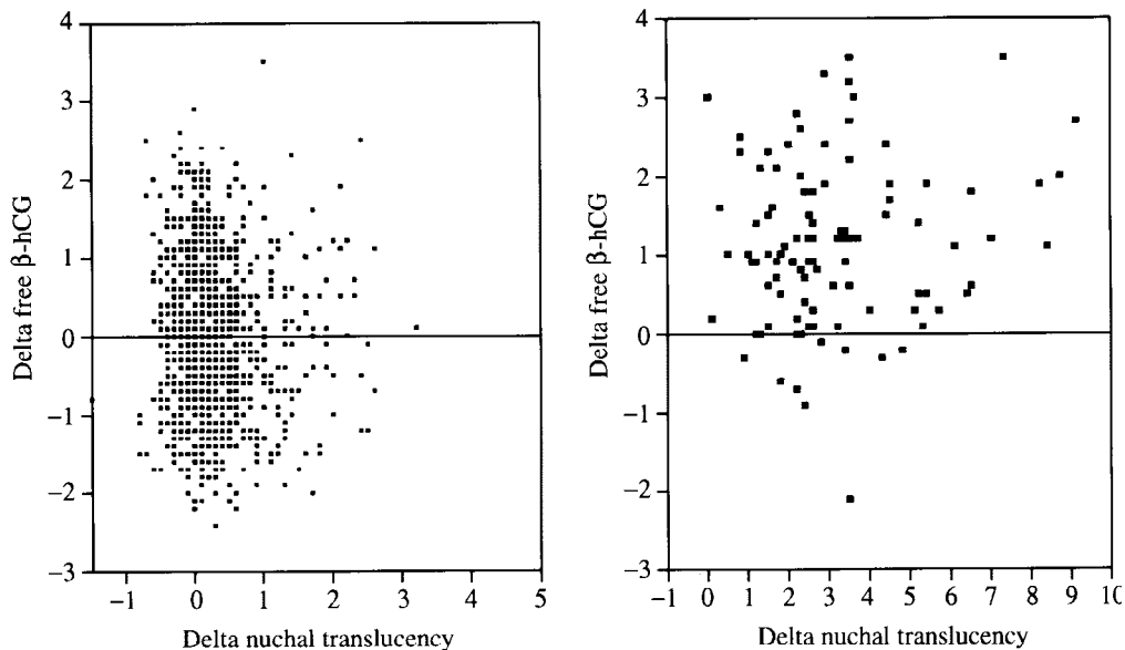
Figure 6 Delta values for maternal serum free \beta -hCG in relation to delta values for fetal nuchal translucency thickness in 2427 normal (left) and 102 trisomy 21 pregnancies (right)
